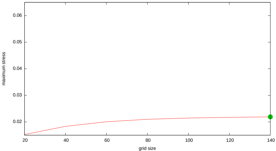
pie_180 Maximum Stress Under Refinement
