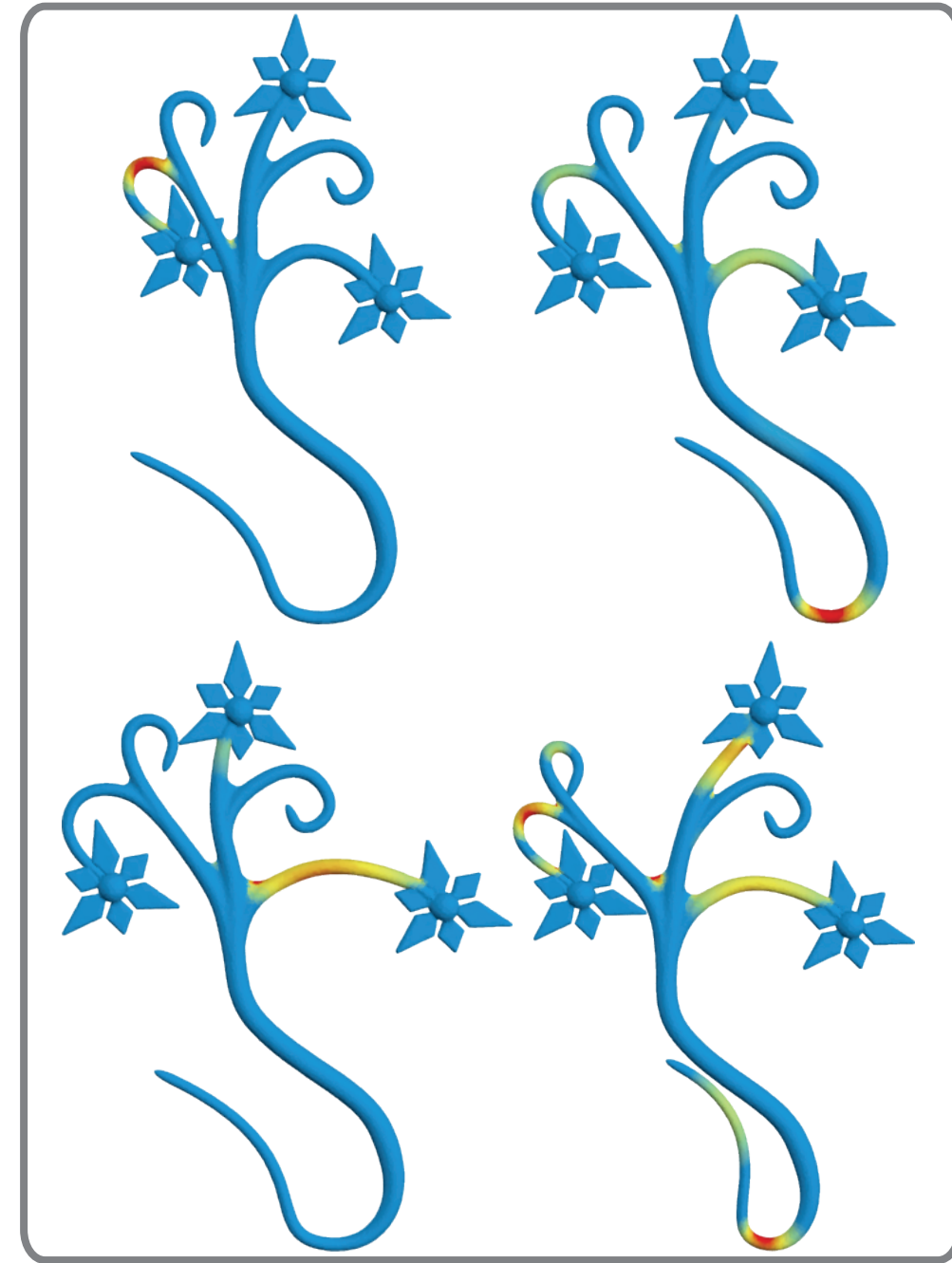
Modal Analysis
