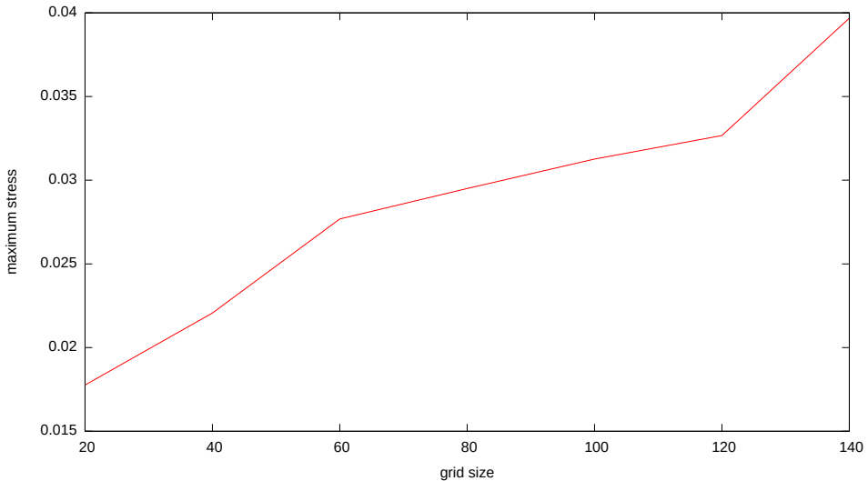
pie_135 Maximum Stress Under Refinement
