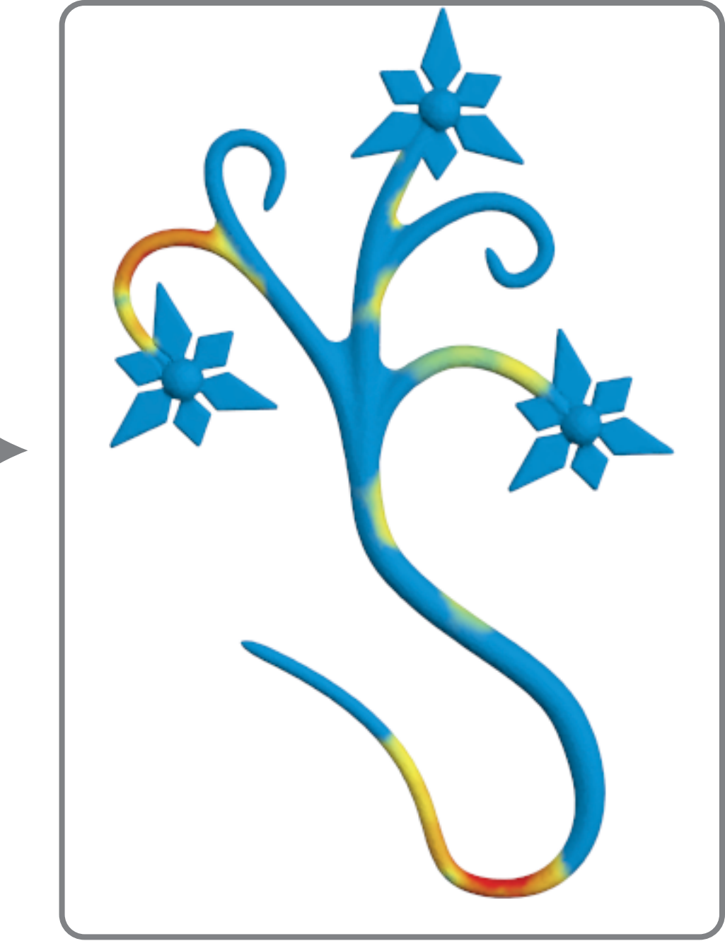
Weakness Map
