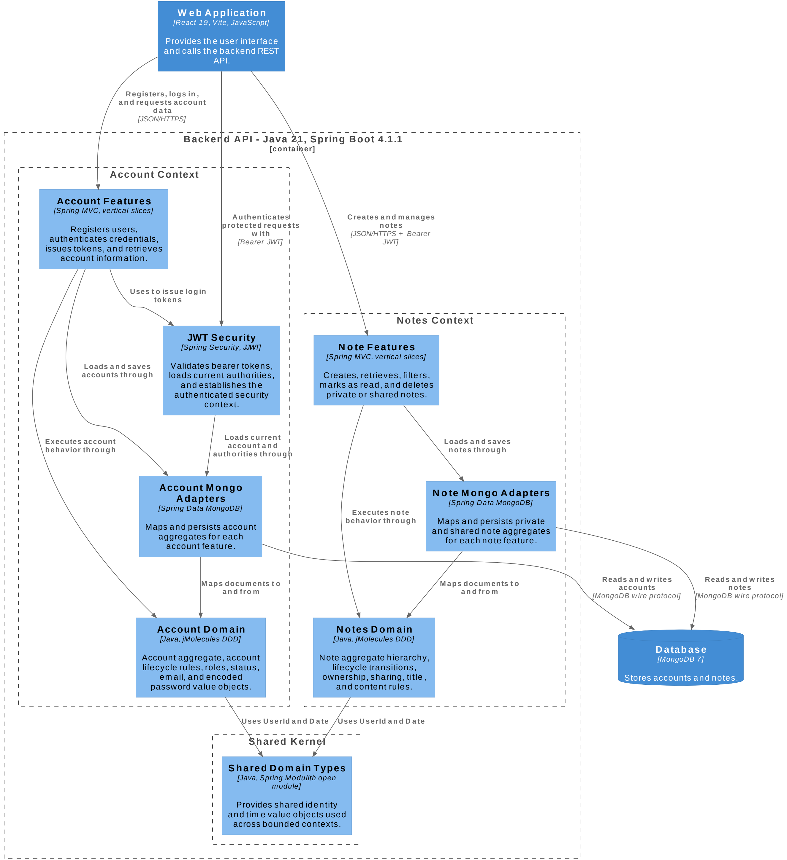
Component diagram for Ghost Notes - Backend API
