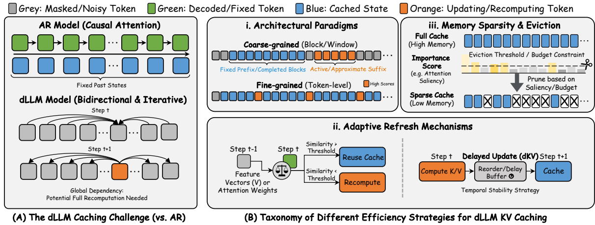
Figure 3: Illustration of Cache Management for dLLMs. (A) The key challenge in dLLM caching. Unlike AR models, dLLMs rely on bidirectional attention and iteratively refine the entire sequence, so KV states are not fixed and cannot be reused. (B) A taxonomy of efficiency strategies for dLLM KV caching: (i) granularity control , from coarse-grained blocks to fine-grained tokens; (ii) adaptive refresh , using similarity thresholds or delayed updates; and (iii) memory sparsity and eviction , guided by saliency signals and budget constraints.
