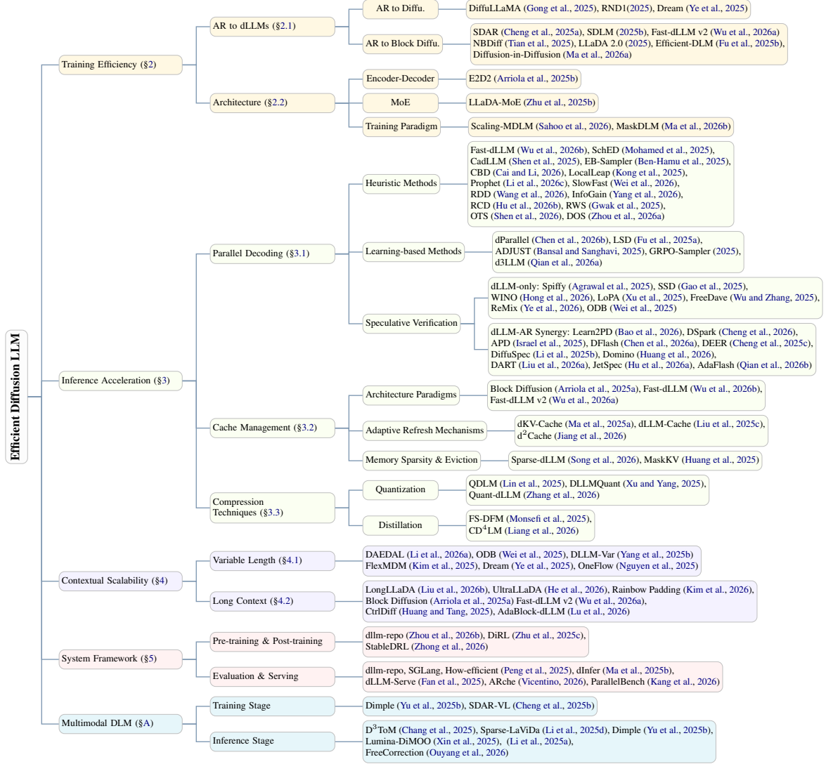
Figure 1: Our taxonomy tree of Efficient Diffusion Language Models (dLLMs).
