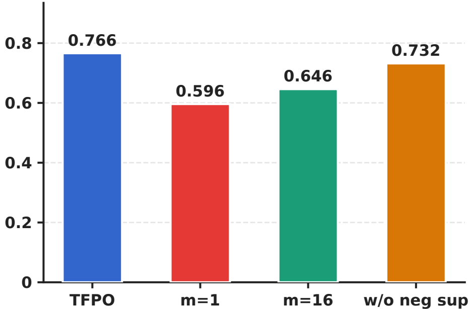
Best MATH500 Accuracy
