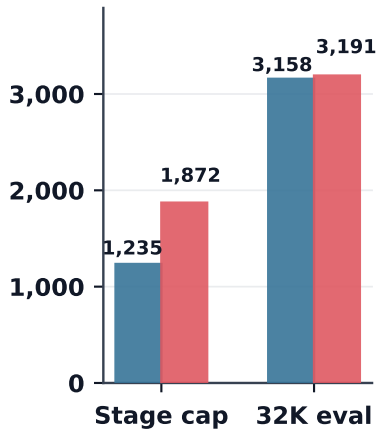
MATH-500
