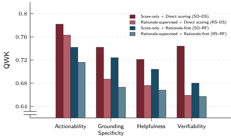
Ordinal tasks
