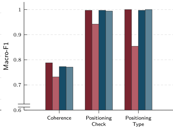
Binary tasks
