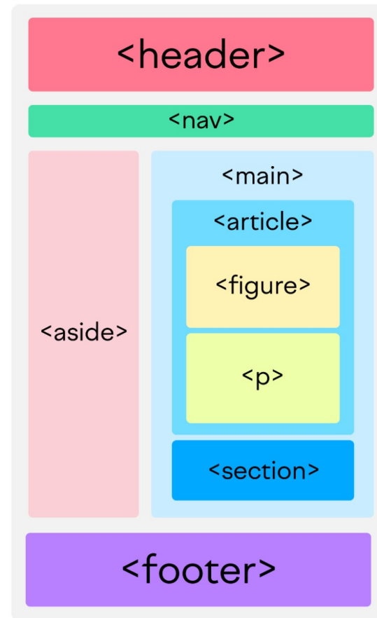
Semantic HTML
