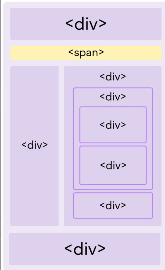
Non-Semantic HTML
