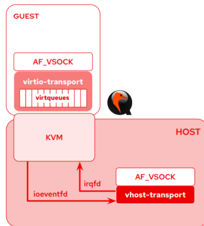
Figure 4: Example of a VSOCK communication structure.
