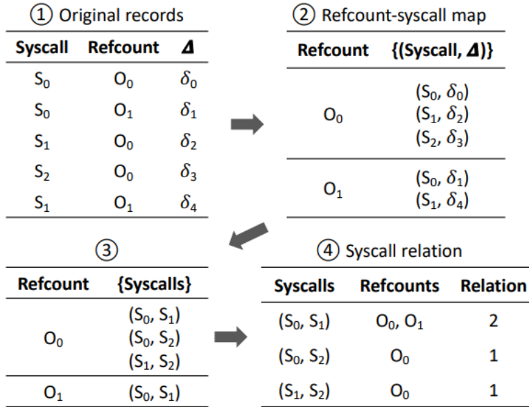
Figure 3: Example of refcount-based syscall relation construction.
