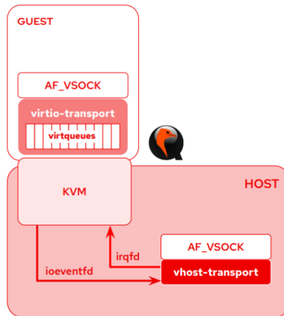
Figure 5: Example of a VSOCK communication structure.
