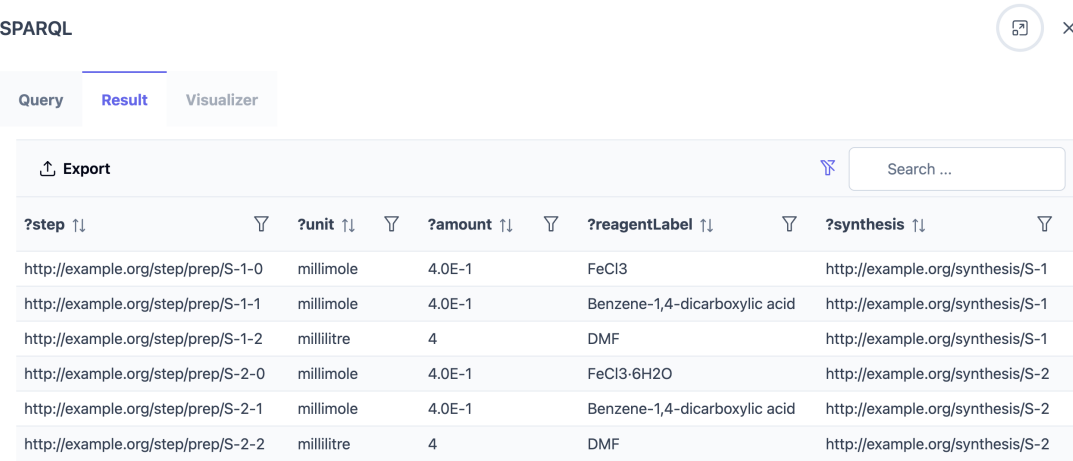
Figure 3.1: Result after running SPARQL query in Figure 3.7.
