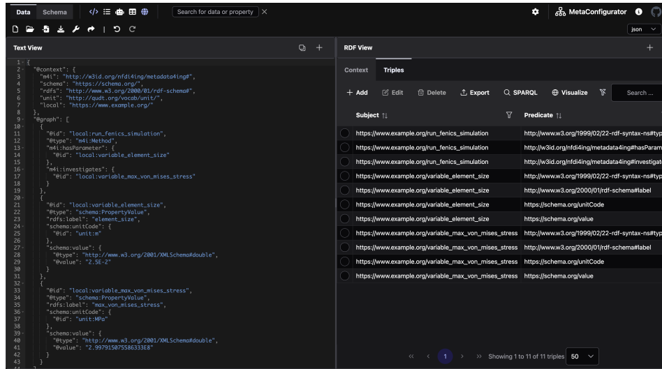
Figure 2.4: JSON-LD output obtained by applying the mapping from Listing 1.7
