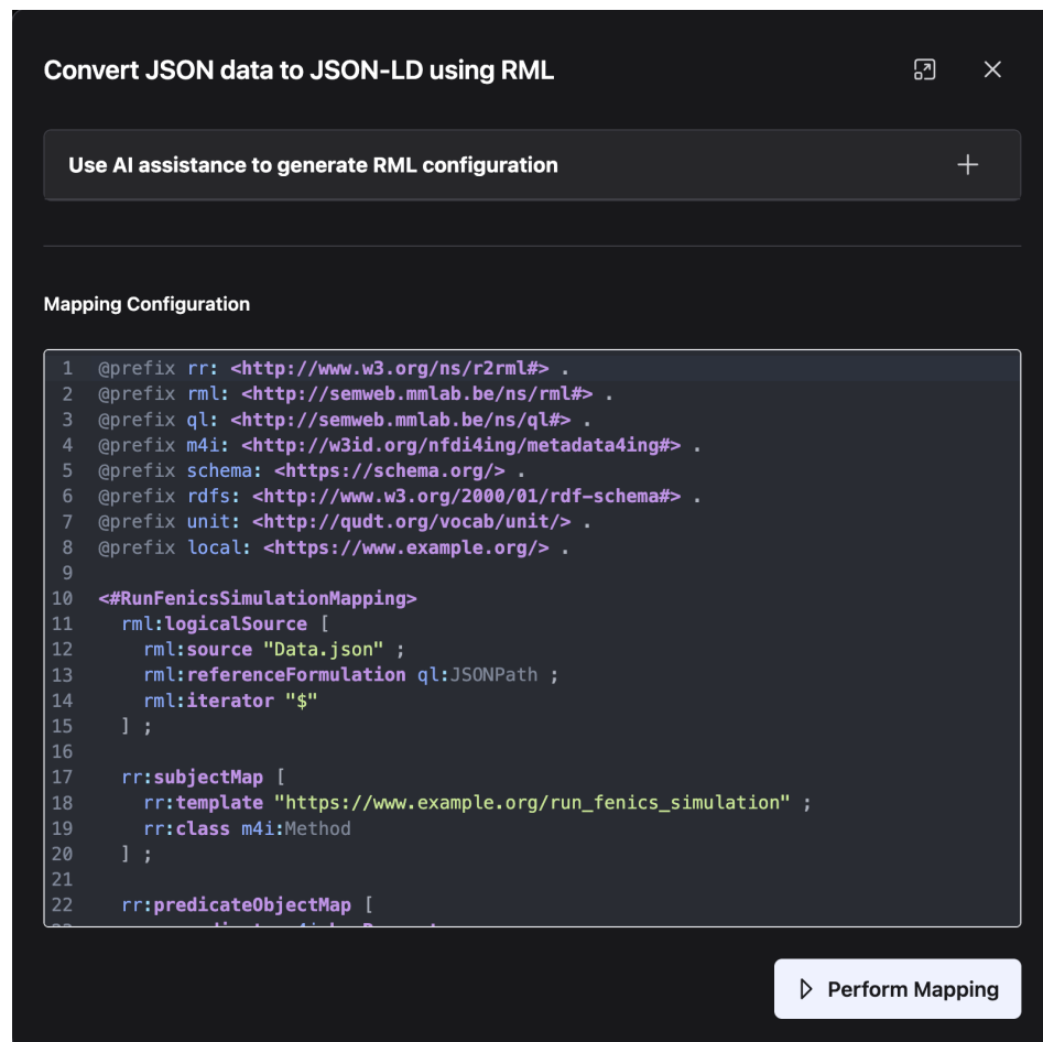
Figure 2.3: AI-generated RML mapping (OpenAI GPT-4o-Mini) based on user-provided hints from Listing 2.1
