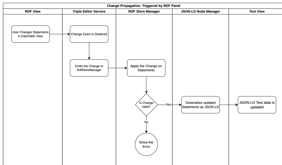
Figure 2.7: Change propagation flow between JSON Text View editor and RDF View, when source of change is the RDF View.
