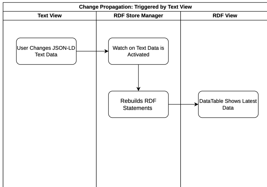
Figure 2.6: Change propagation flow between JSON Text View editor and RDF View, when source of change is the JSON editor.
