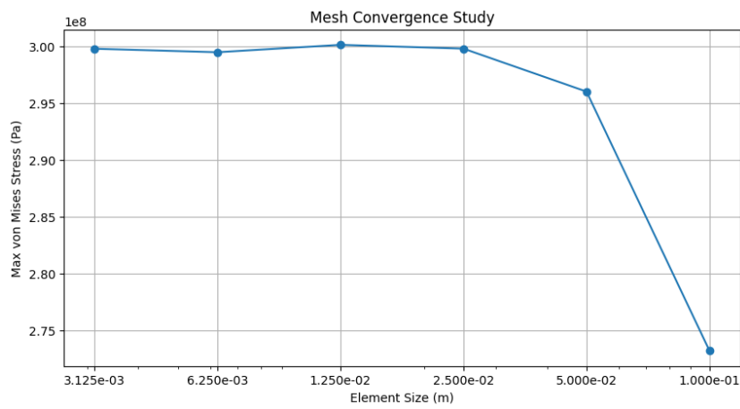
Figure 2.10: Data exported as CSV could be visualized as a plot of element size vs. maximum von Mises stress, revealing trends in the simulation results.
