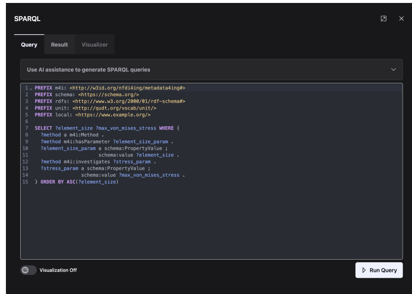
Figure 2.8: SPARQL query editor with AI-generated query based on user hints.
