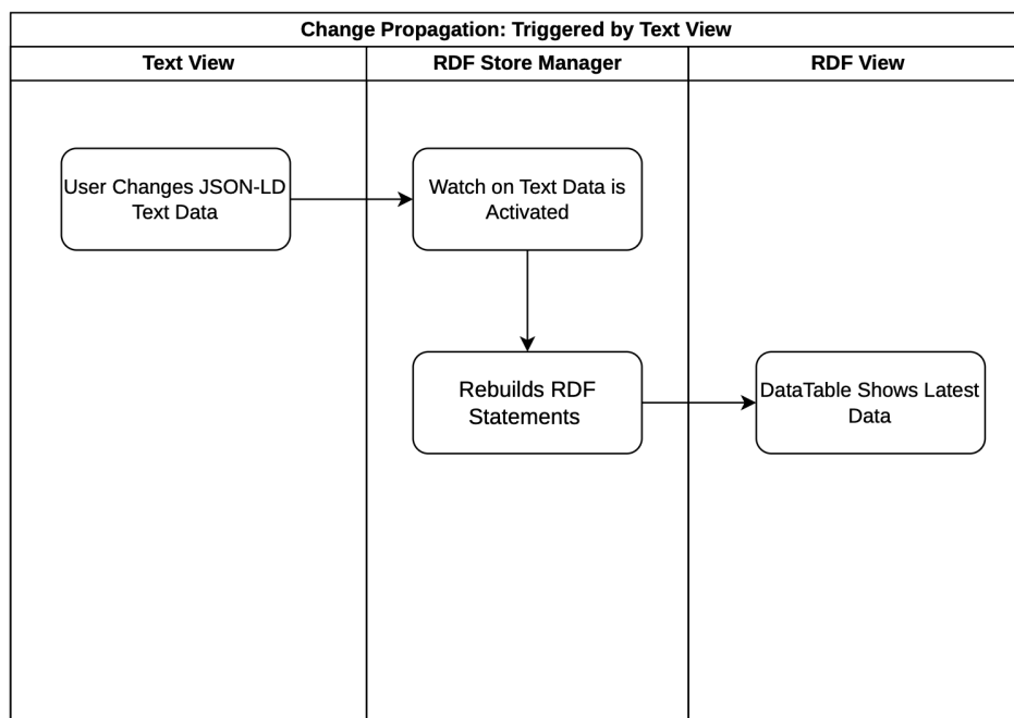
Figure 2.6: Change propagation flow between Text View and RDF View when the source of change is the Text View.
