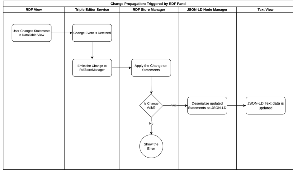
Figure 2.7: Change propagation flow between Text View and RDF View when the source of change is the RDF View.
