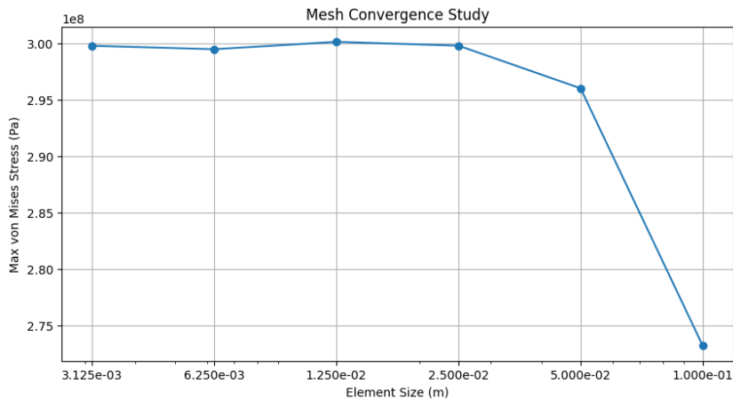
Figure 2.9: Data exported as CSV could be visualized as a plot of element_size vs. max_von_mises_stress , revealing trends in the simulation results.
