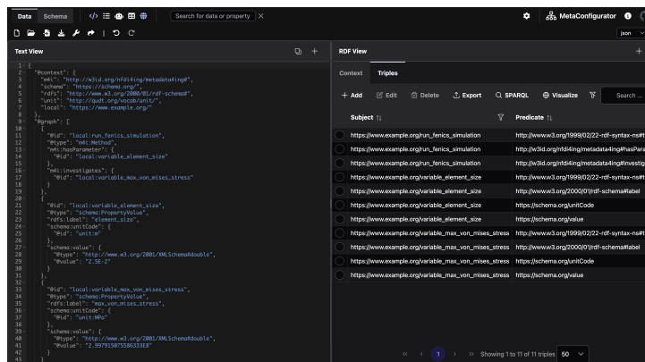
Figure 2.5: JSON-LD output obtained by applying the mapping from Listing 1.7, focused on the Triples tab.
