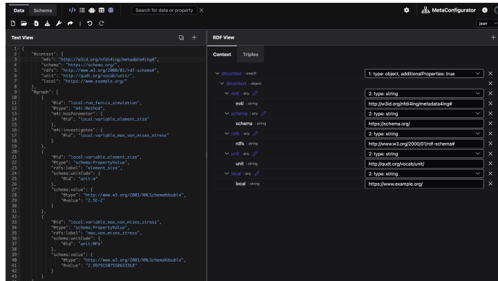
Figure 2.4: JSON-LD output obtained by applying the mapping from Listing 1.7, focused on the Context tab.
