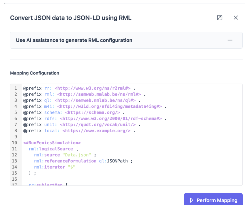
Figure 2.3: AI-generated RML mapping based on user-provided hints from Listing 2.2.
