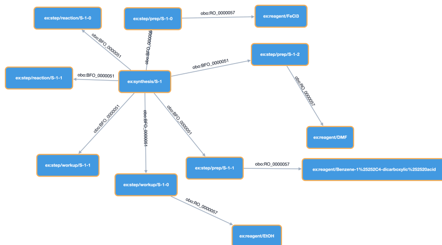
Figure 3.2: Knowledge graph visualization of the JSON-LD data in Listing 3.5, rendered in the Visualization dialog.
