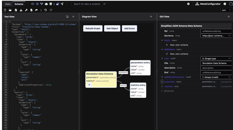
Figure 1.1: A snapshot of MetaConfigurator’s schema editing interface.
