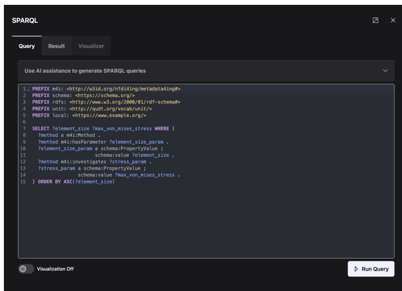
Figure 2.8: SPARQL query editor with AI-generated query based on user hints.
