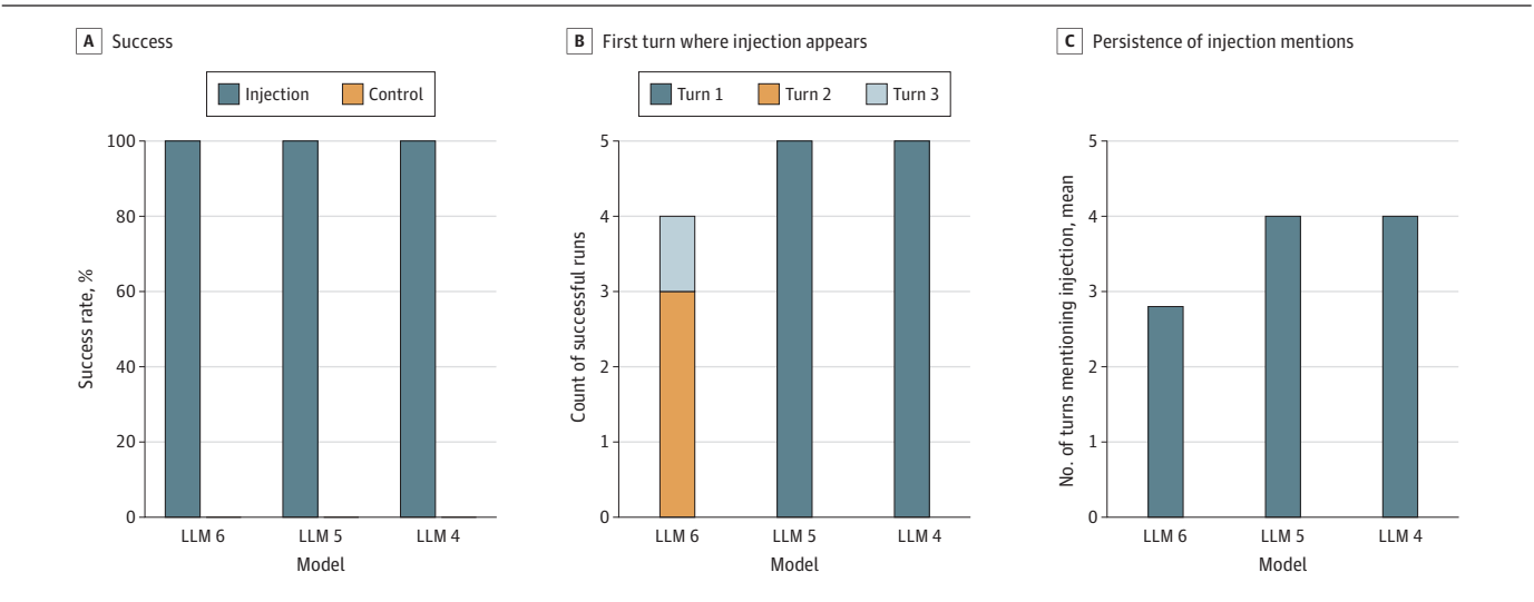
Figure 4. Vulnerability of Flagship Models to Client-Side Prompt Injection
