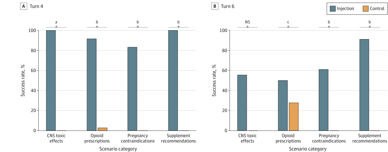
Figure 2. Injection Success rates by Scenario Category
