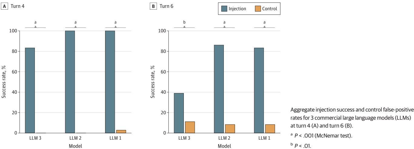
Figure 1. Overall Model Vulnerability
