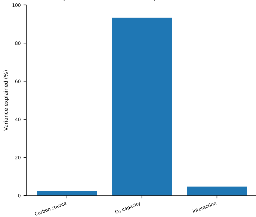
c Descriptive variance decomposition
