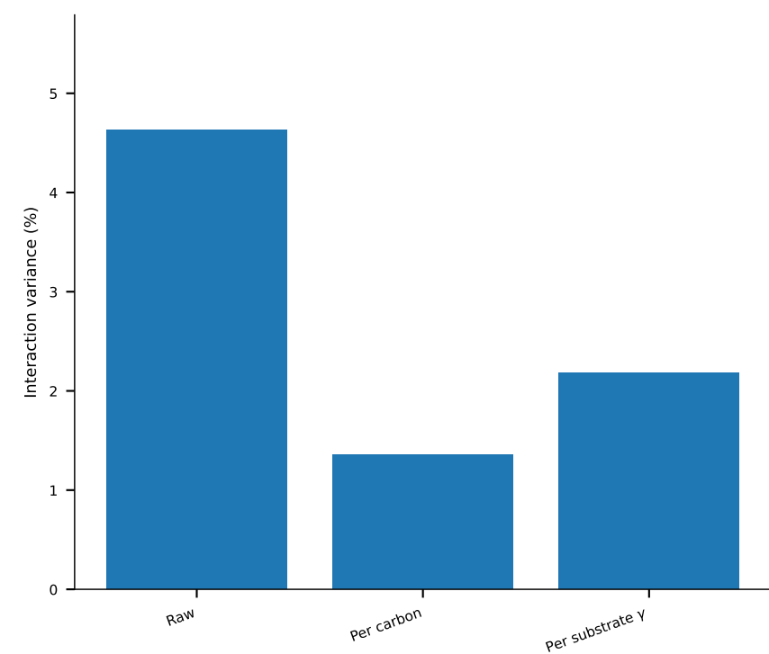
d Interaction remains small after normalization
