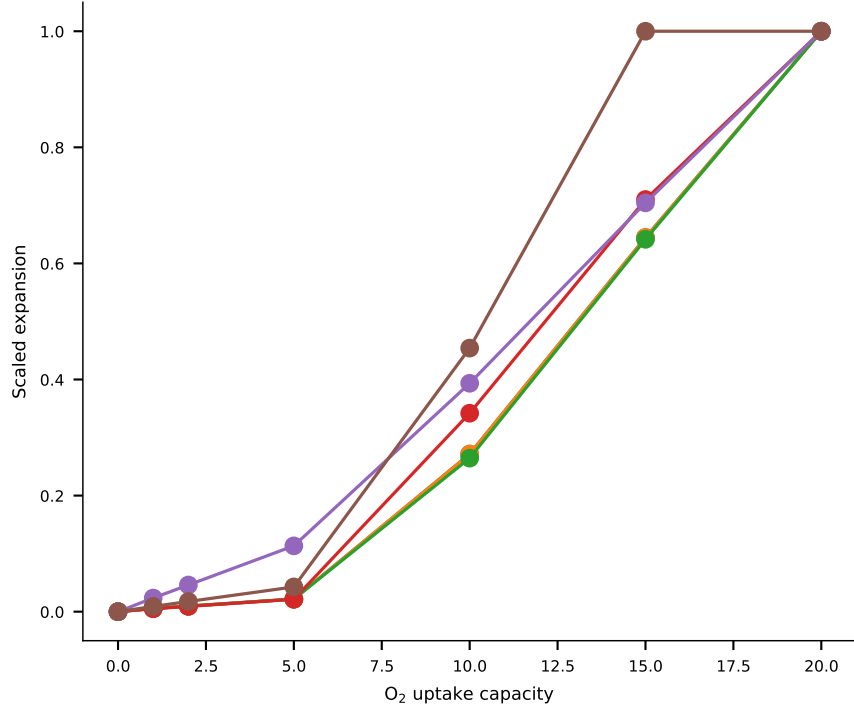
d Interaction remains small after normalization
