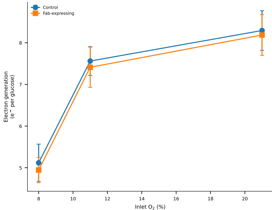
a Electron generation per glucose falls with oxygen restriction
