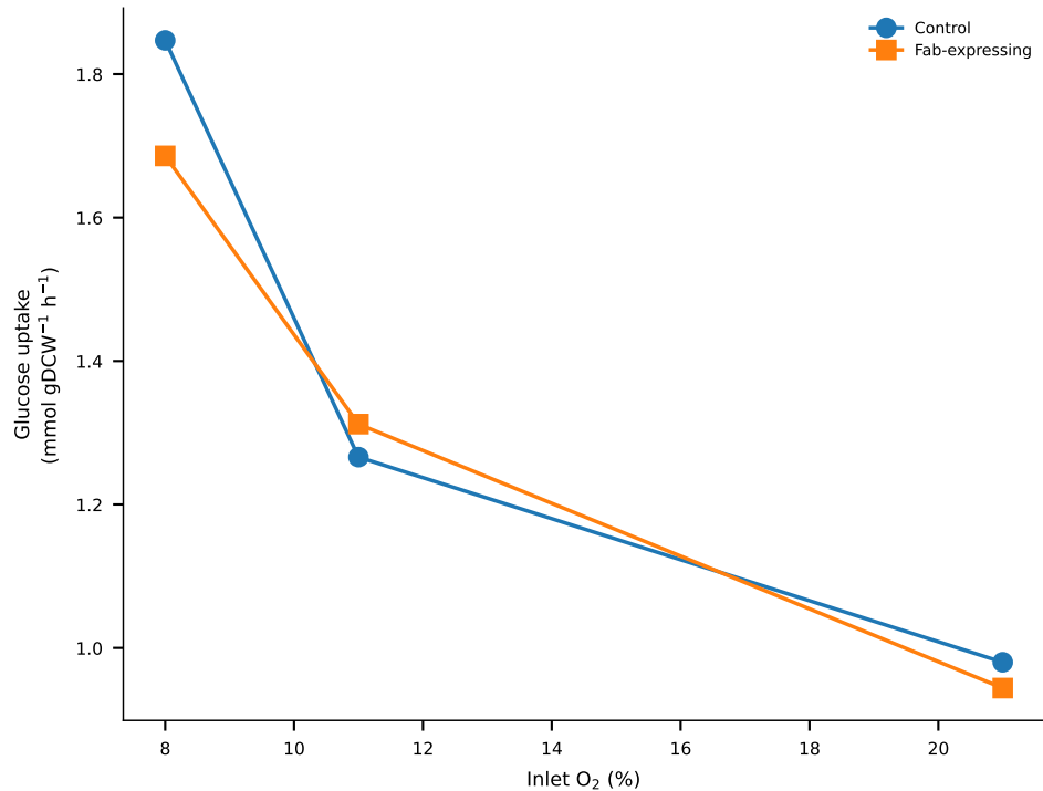
b Glucose uptake rises as oxygen is restricted
