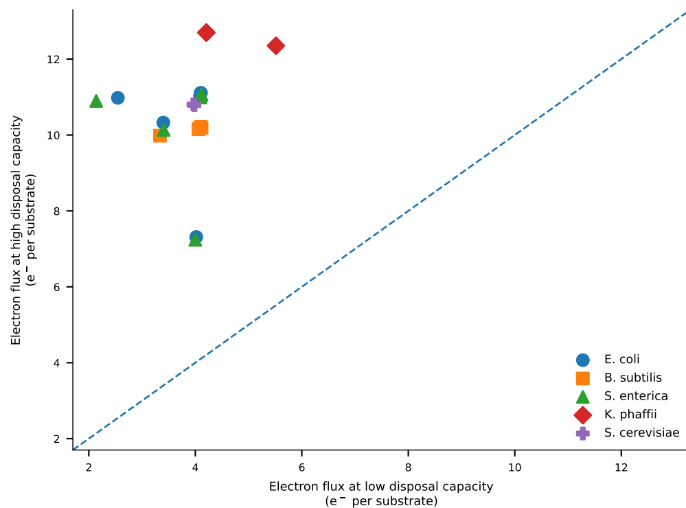
c Baseline variation after reducing-power normalization
