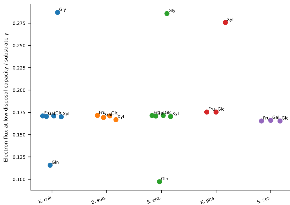
c Baseline variation after reducing-power normalization
