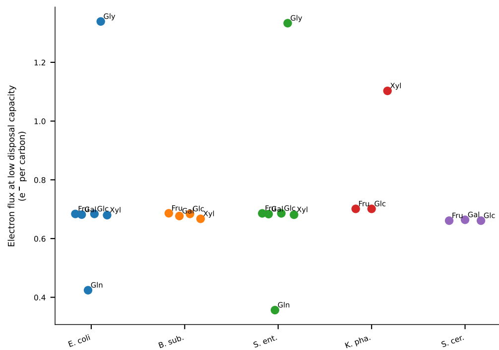
b Baseline variation after carbon normalization
