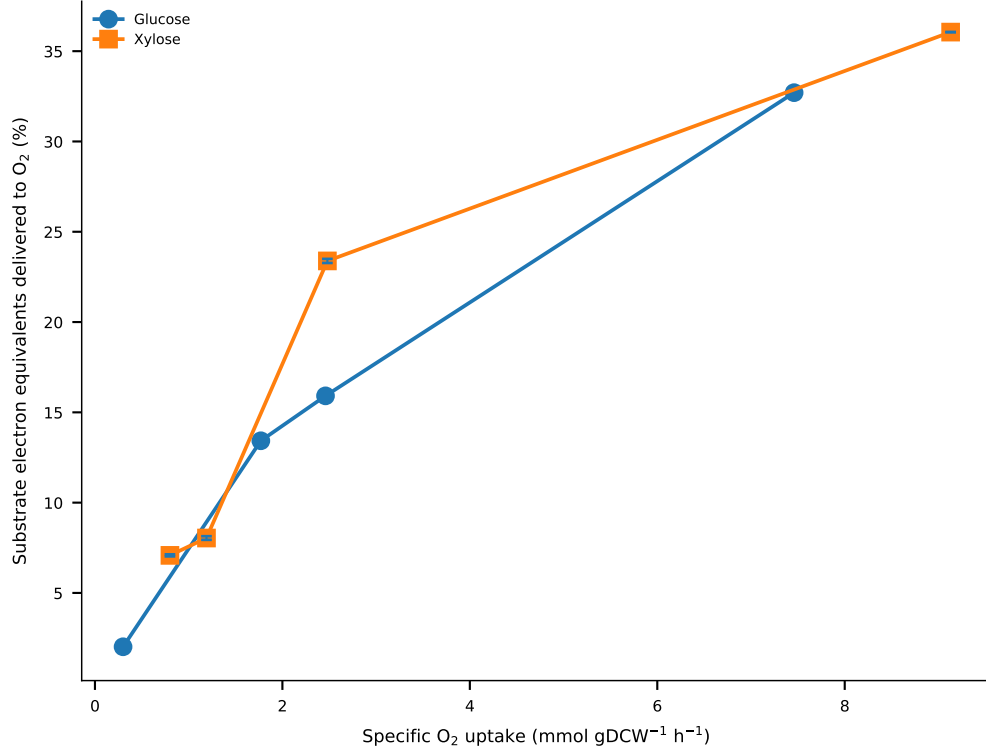
a Electron delivery to oxygen rises on both carbon sources
