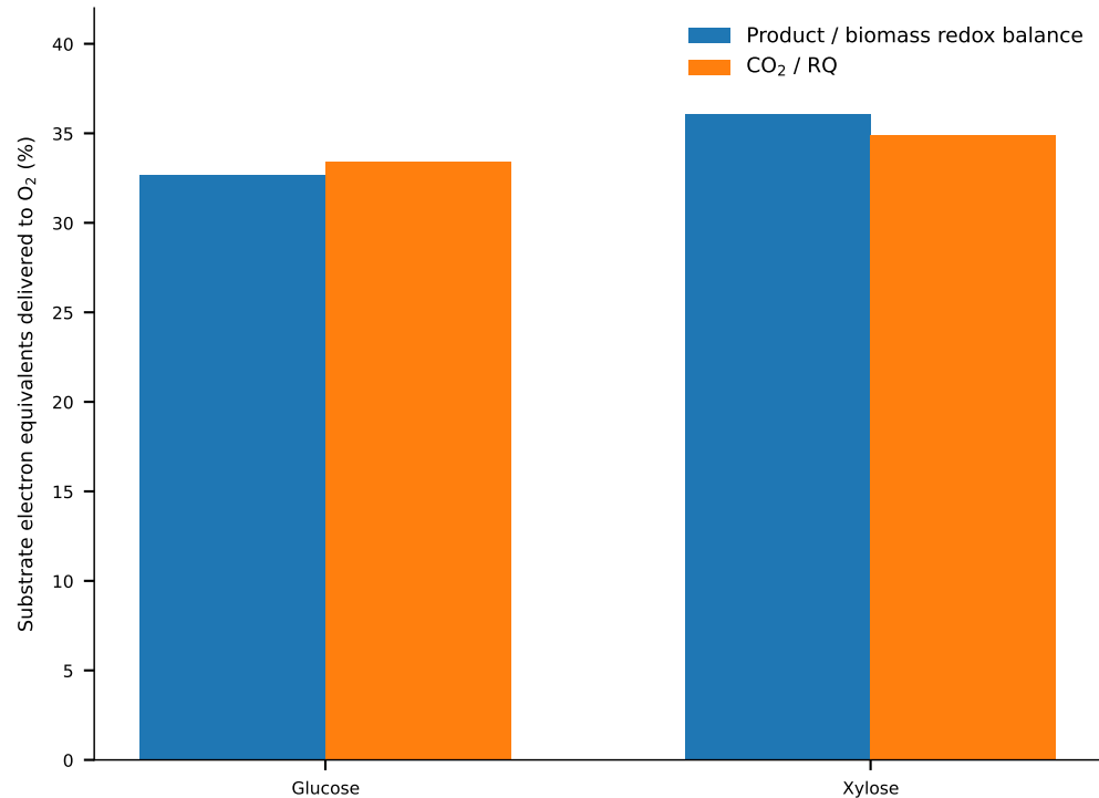
b Aerobic balance agrees with an independent RQ estimate
