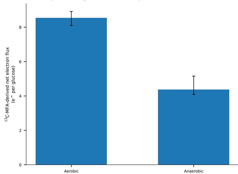
d Independent glucose flux maps
