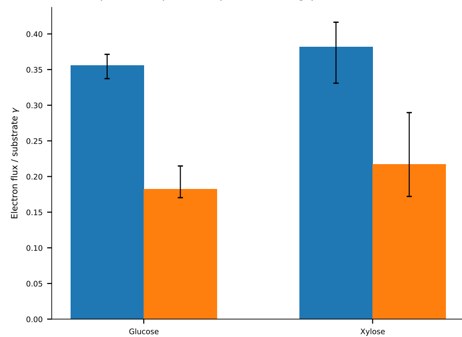
c Compression persists per reducing power
