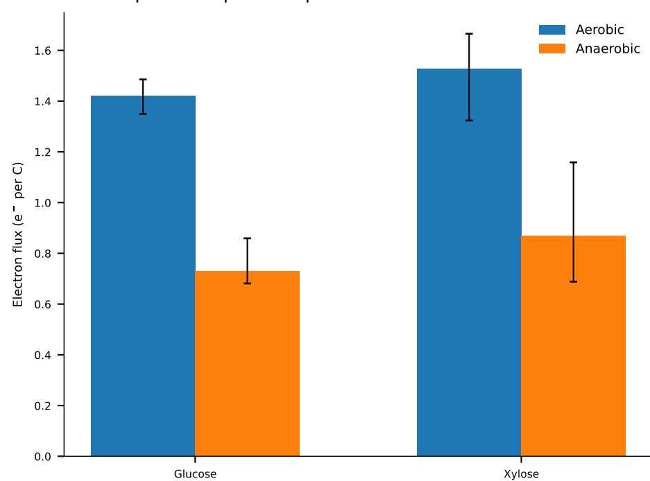
b Compression persists per carbon
