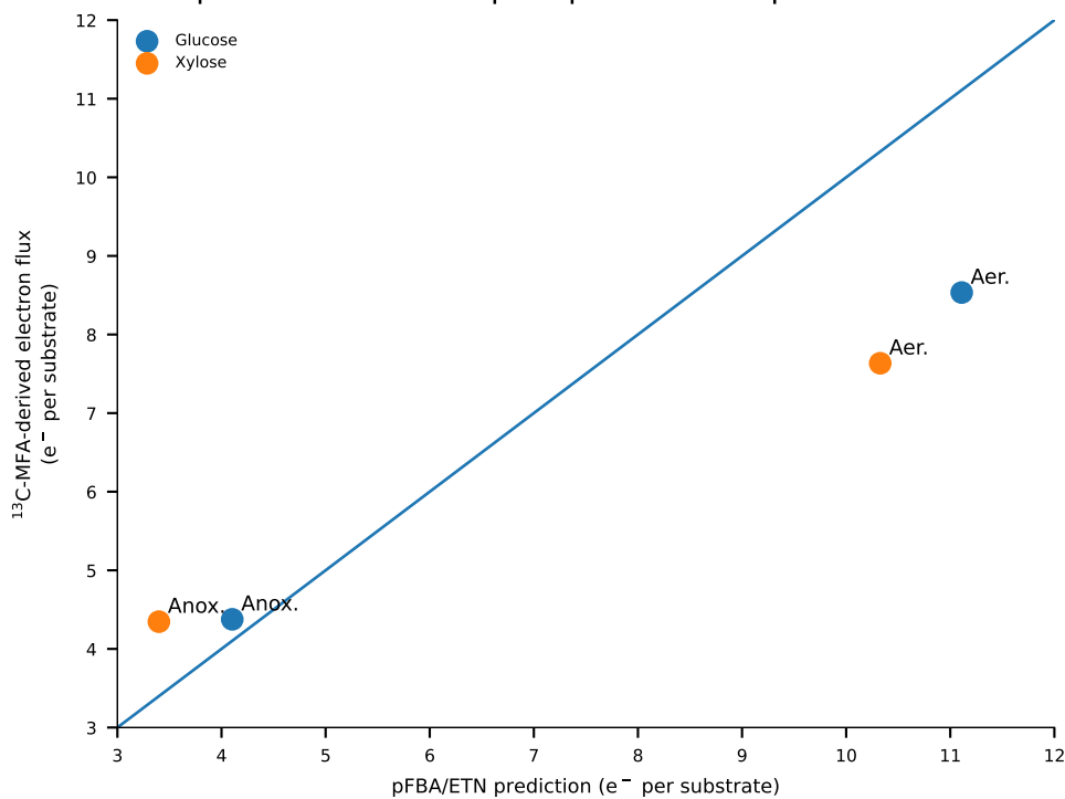
c Compression persists per reducing power
