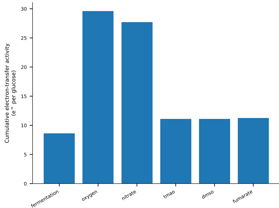
b Relay can increase before net flux
