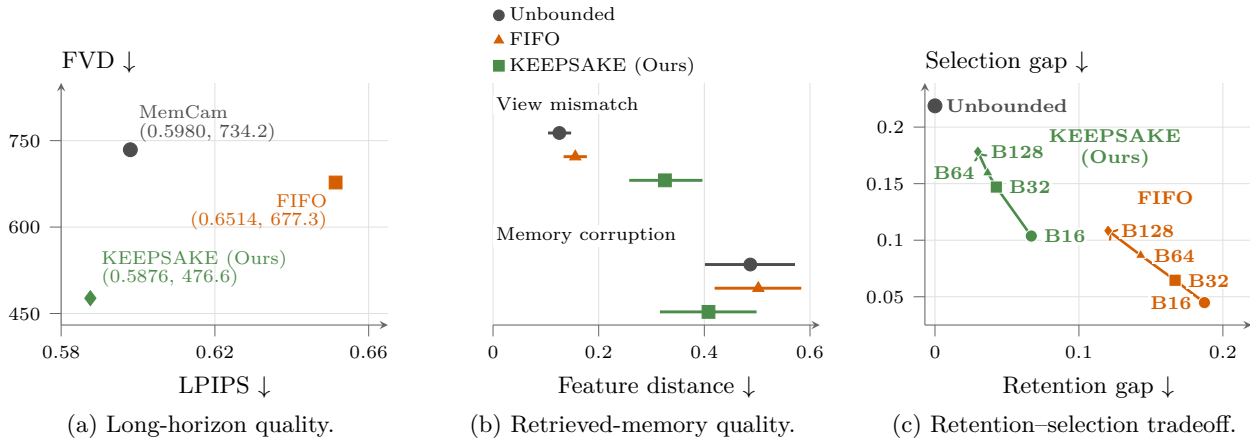
Figure 1: Generation quality and memory diagnostics. (a) Fifteen matched 180-second MemCam rollouts; bounded methods use B = 32 . (b) Mean view mismatch and memory corruption on fifteen matched 60-second rollouts, using common baseline pixels and DINOv2 cosine distance; FIFO and KEEPSAKE use B = 32 ; whiskers show 95% trajectory-bootstrap intervals. (c) Original thirteen-trajectory, 180-second retention-selection analysis; labels denote memory budgets. Lower is better on both axes.
