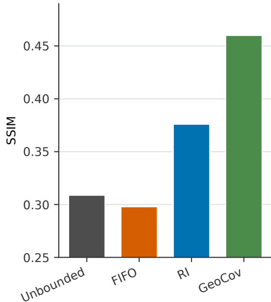
Same-video selected SSIM
