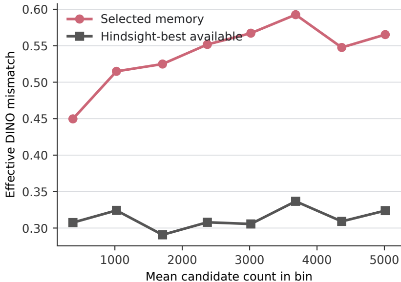
Selected evidence worsens; best available stays flat
