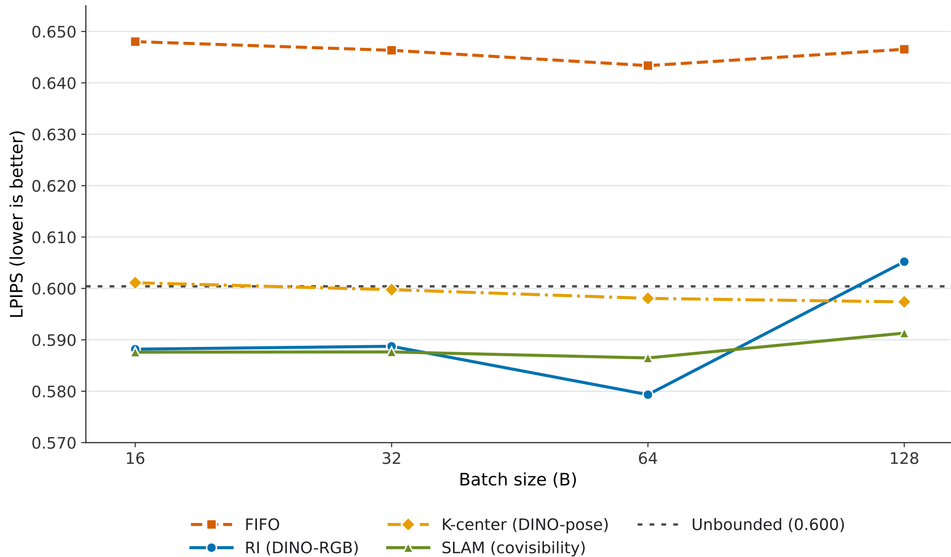
LPIPS vs. Batch Size (180 s)
