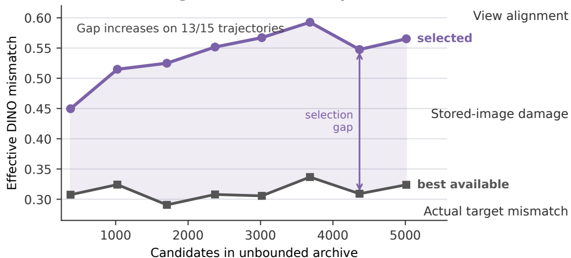
(a) Selected degrades; available stays stable
