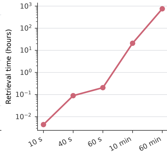
Quadratic search growth
