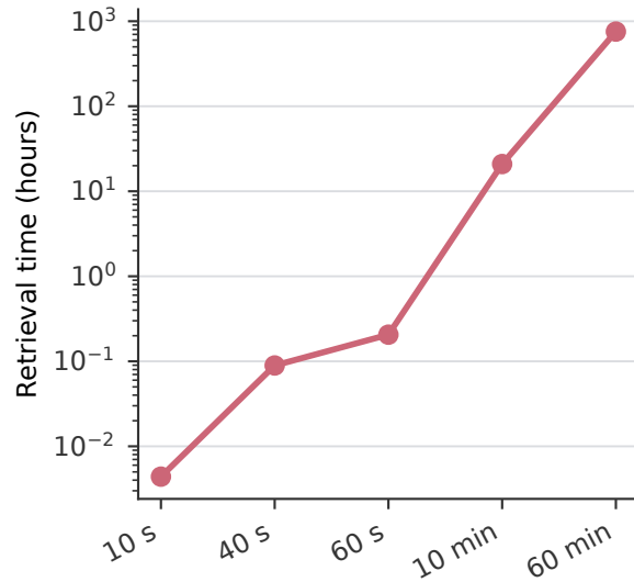
Quadratic search growth
