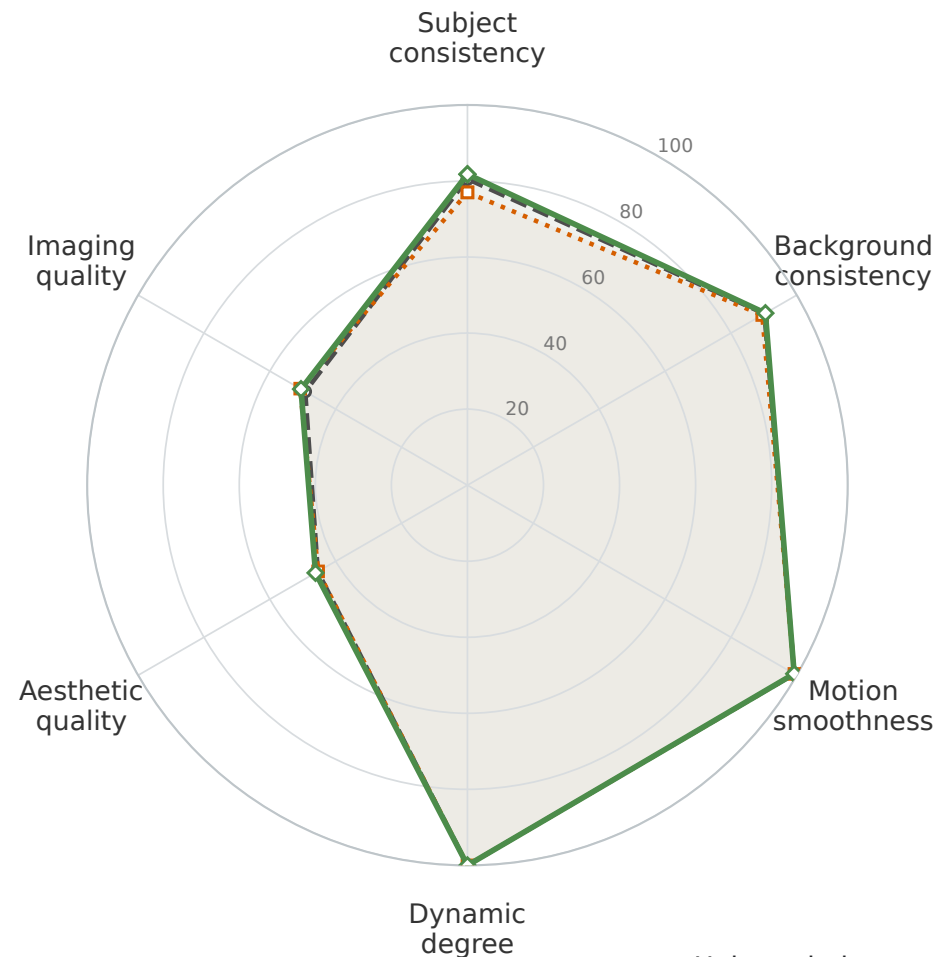
(a) VBench
