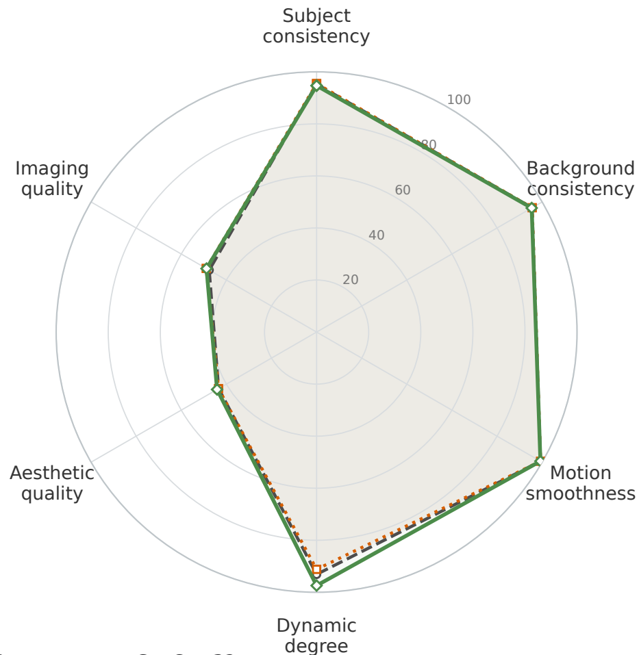
(b) VBench-Long
