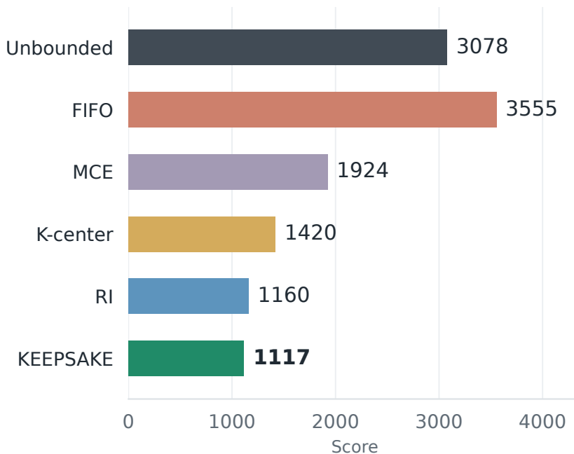
FVD / lower is better
