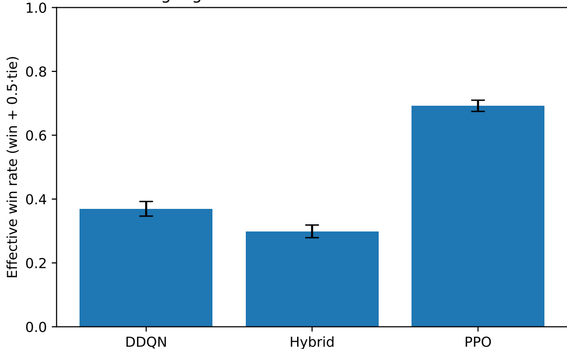
Training-log based effective win rates with 95% CI
