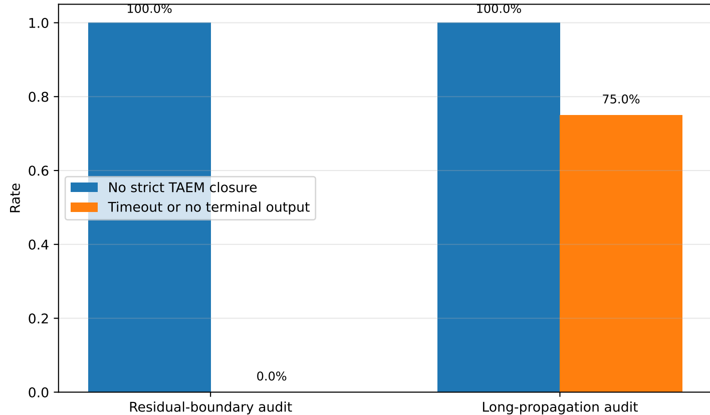
Boundary-diagnostic summary
