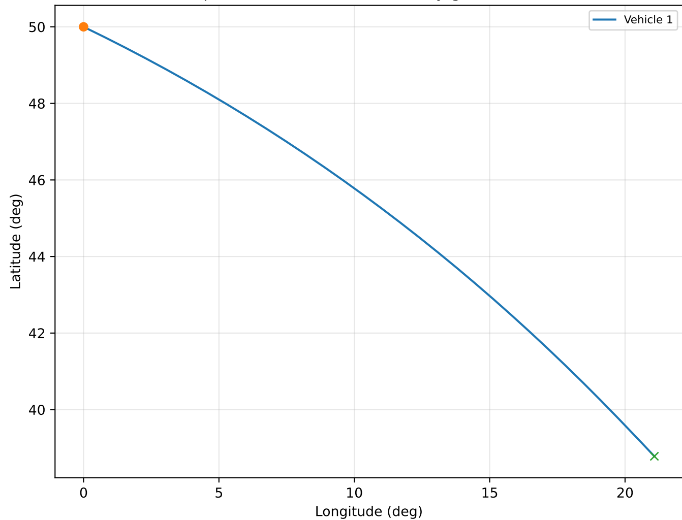
Representative failure-boundary ground track
