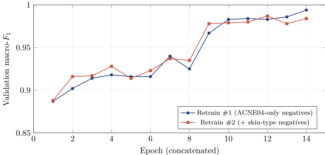
Skin-conditions retrain: macro- F_1 per epoch
