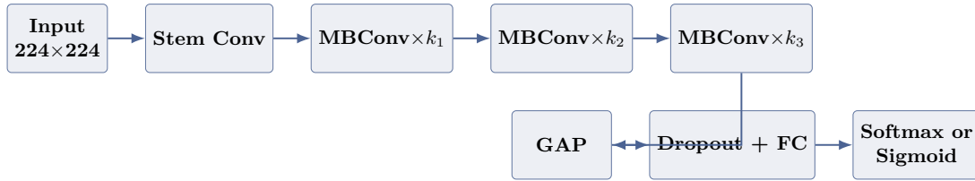
Figure 3.1: Schematic of the EfficientNet-B0 backbone used for each of CARA’s three classifiers. The classifier head (dropout + fully-connected + softmax or sigmoid) is the only part re-initialised for each task.
