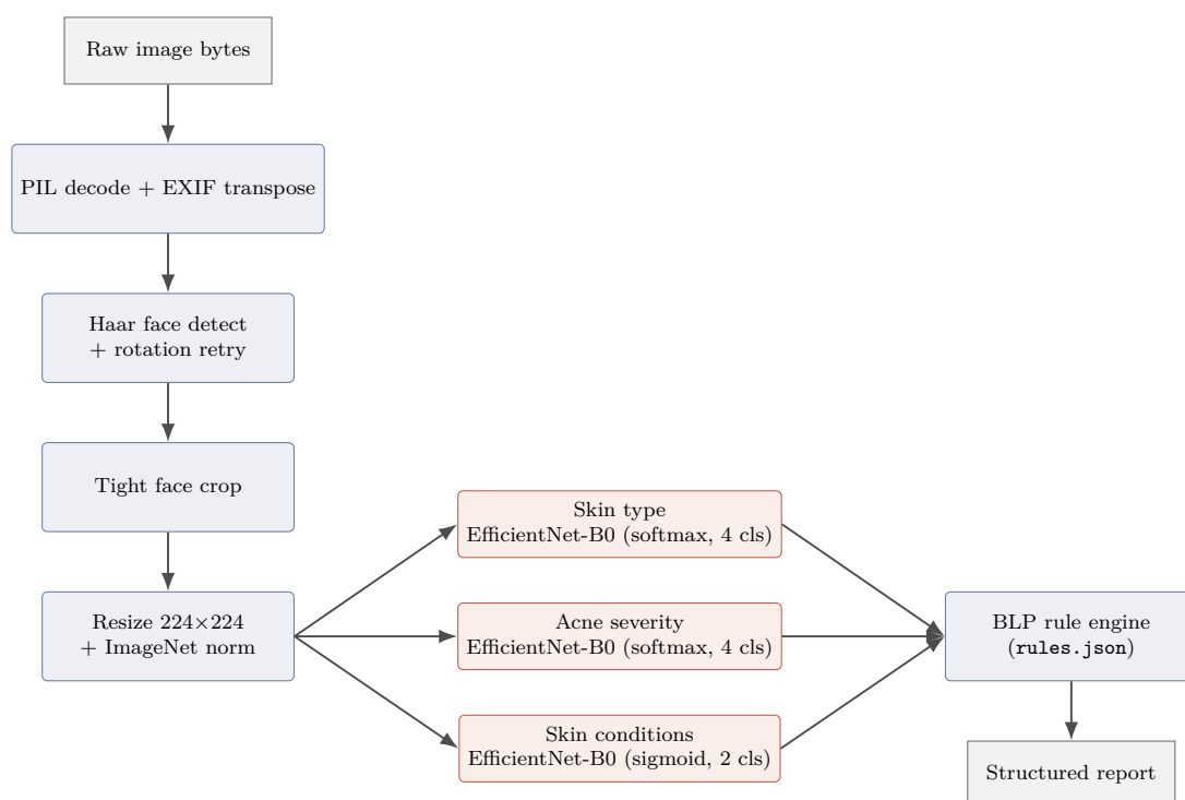
Figure 5.1: End-to-end runtime pipeline used by CARA at submission time. The three EfficientNet-B0 models run sequentially on a shared preprocessed tensor; the BLP engine composes their outputs deterministically. Each of the arrows in the diagram was, at one point in Phase 3, either wrong or missing.
