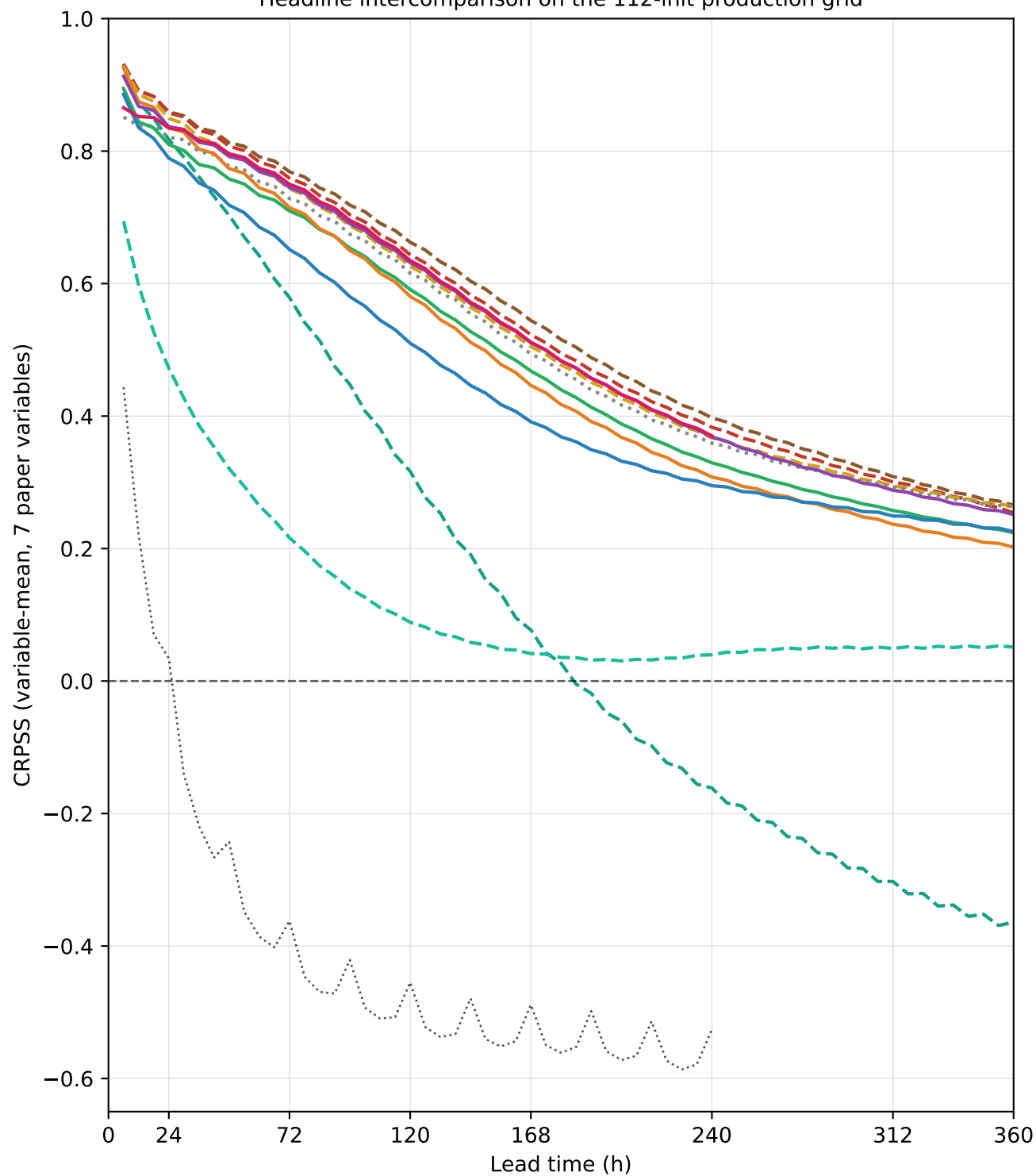
Headline intercomparison on the 112-init production grid
