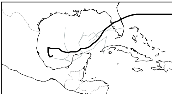
04 00 UTC IFS-ENS (7/10)
