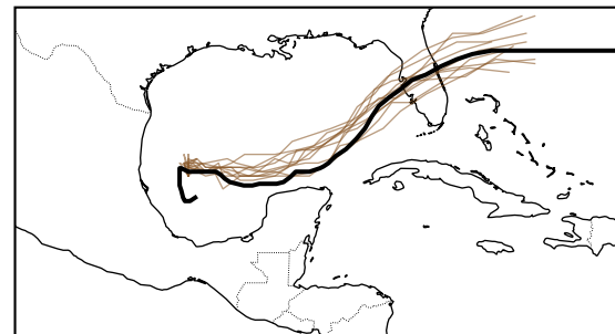
06 00 UTC AIFS-ENS (10/10)
