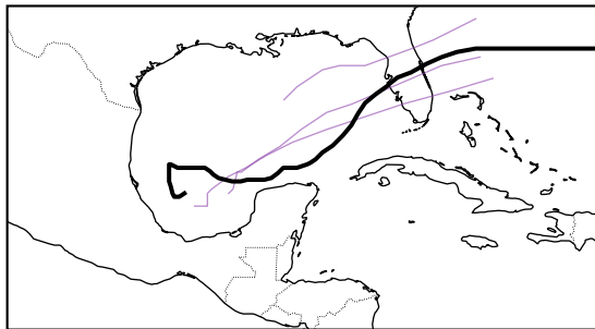
AIFS (weight+IC) (3/10)
