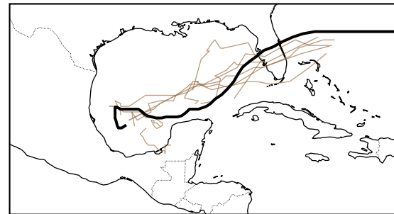
AIFS-ENS (8/10)
