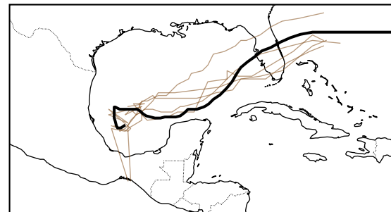
04 00 UTC AIFS-ENS (5/10)
