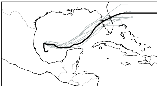
06 00 UTC IFS-ENS (9/10)
