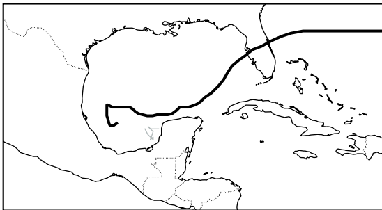
IFS-ENS (1/10)
