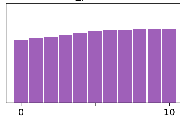
aifs_perturbed
