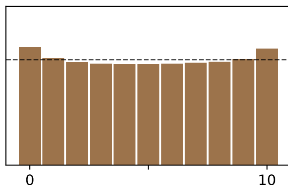
AIFS-ENS
