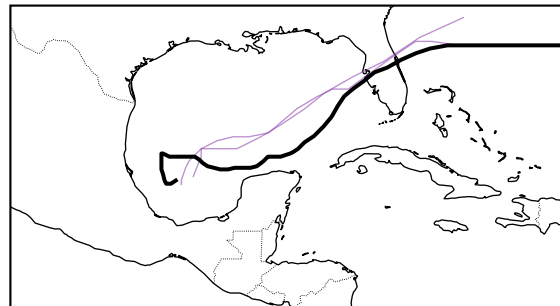
AIFS (weight+IC) (2/10)
