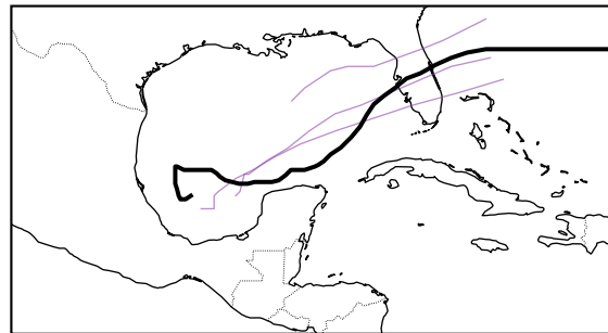
AIFS (weight+IC) (3/10)
