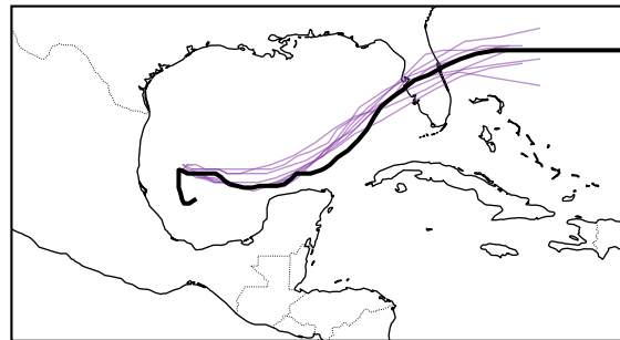
AIFS (weight+IC) (8/10)
