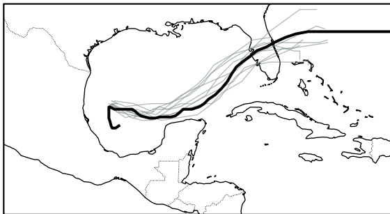
IFS-ENS (9/10)
