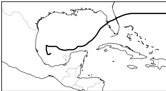
IFS-ENS (1/10)
