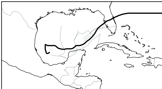
IFS-ENS (7/10)
