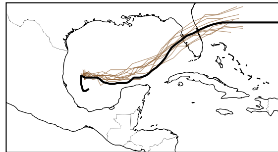
AIFS-ENS (10/10)
