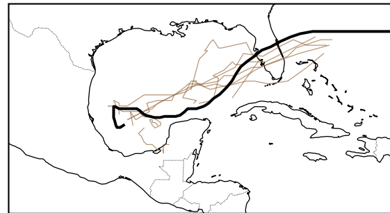
AIFS-ENS (8/10)
