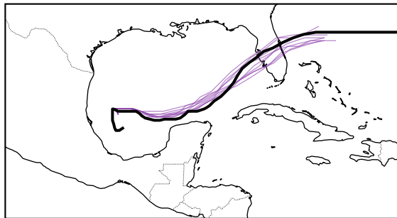
AIFS (weight-only) (9/10)
