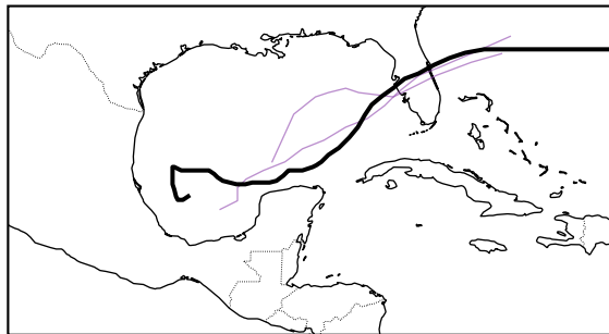
AIFS (weight-only) (2/10)
