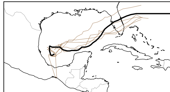
AIFS-ENS (5/10)
