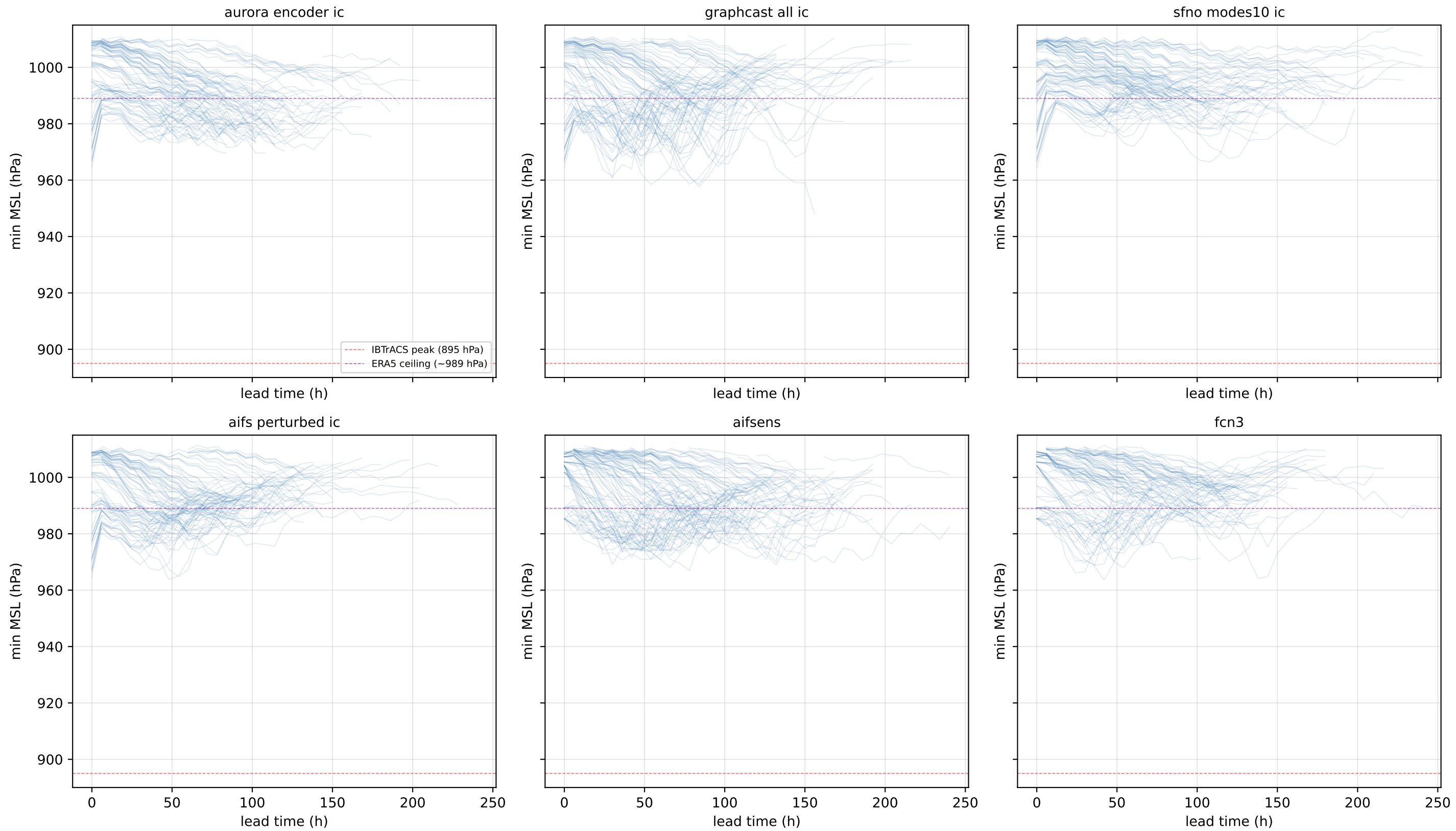
Hurricane Milton MSL minimum vs lead time, per baseline (each line = one member from one init)
