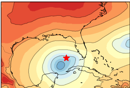
init 05/10 12Z, lead 96h
