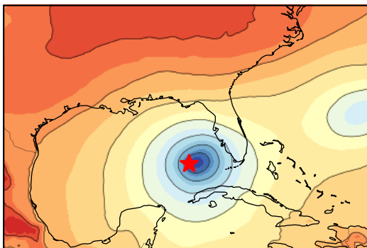
init 06/10 12Z, lead 72h
