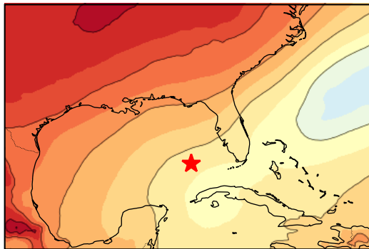
init 03/10 12Z, lead 144h
