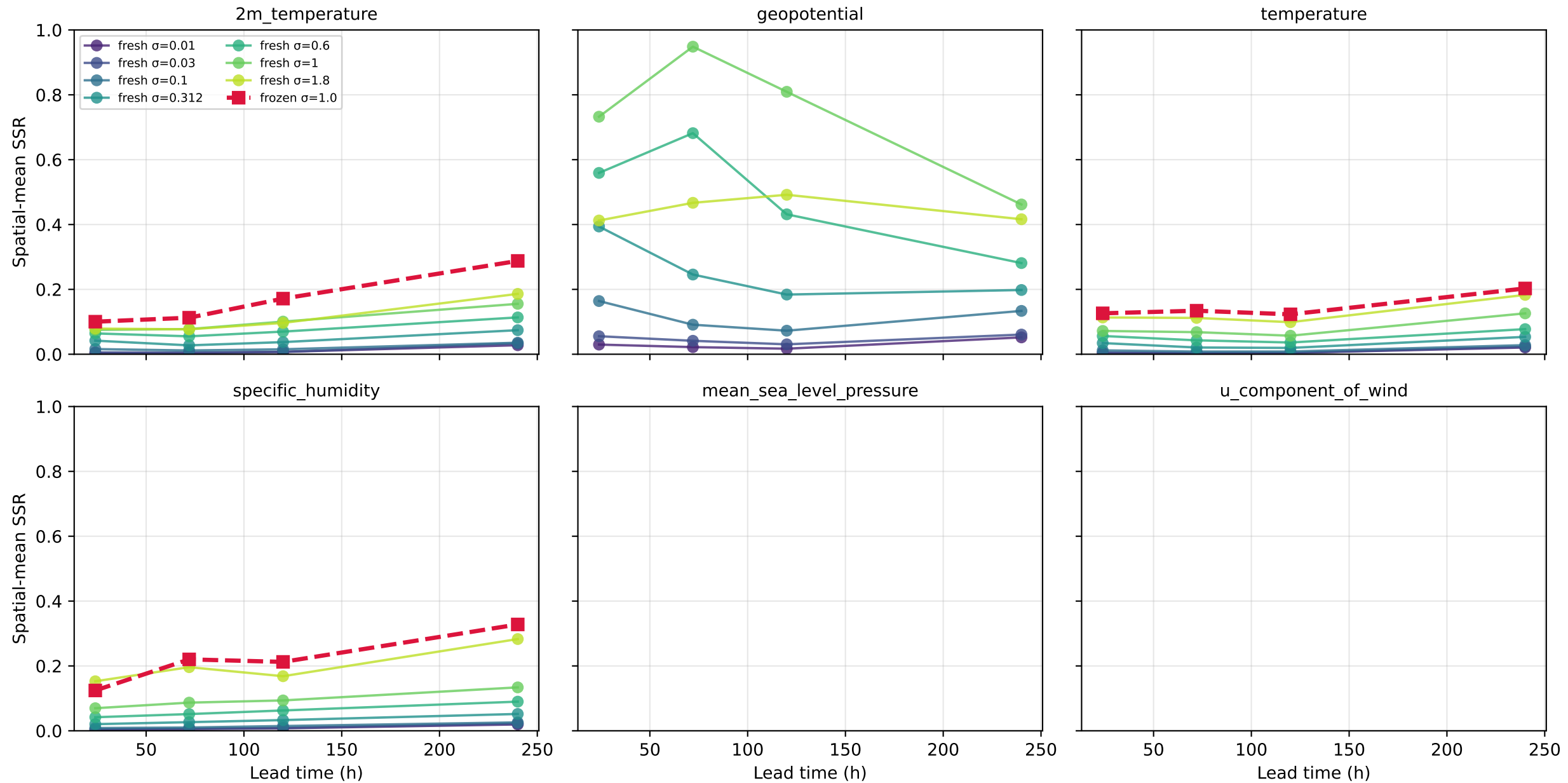
Phase 6a: Spatial-mean SSR -- fresh-per-step vs frozen (GraphCast n_coarse=42)
